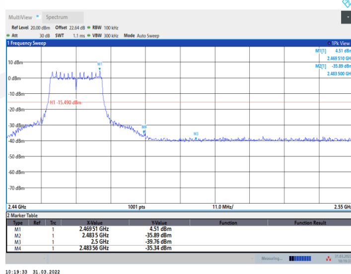
11G_Ant2_High_2462
