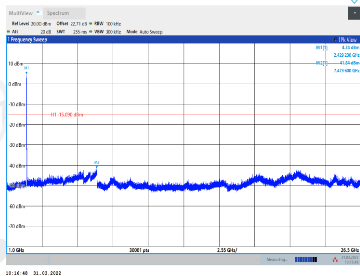
11G_Ant2_2437_0~Reference
