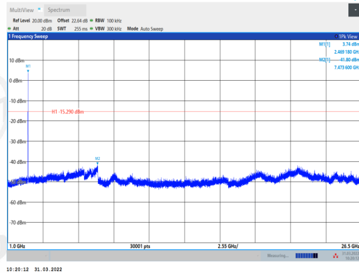
11G_Ant2_2462_0~Reference
