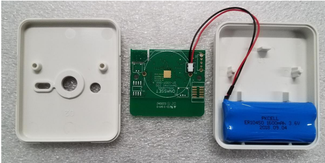
PCB Image Side B
