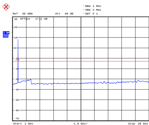
LTE Band 4 1.4MHz CH- High 1GHz ~20GHz
