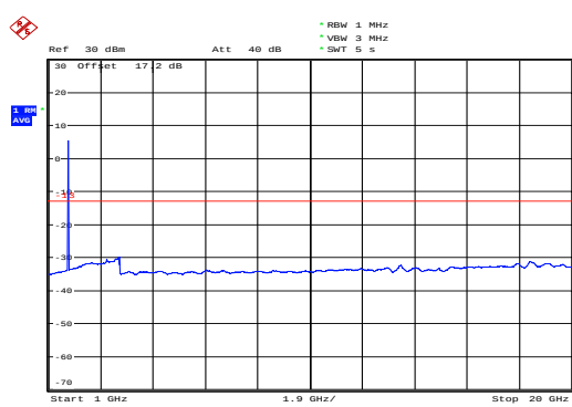
LTE Band 4 1.4MHz CH-Low 1GHz ~20GHz
