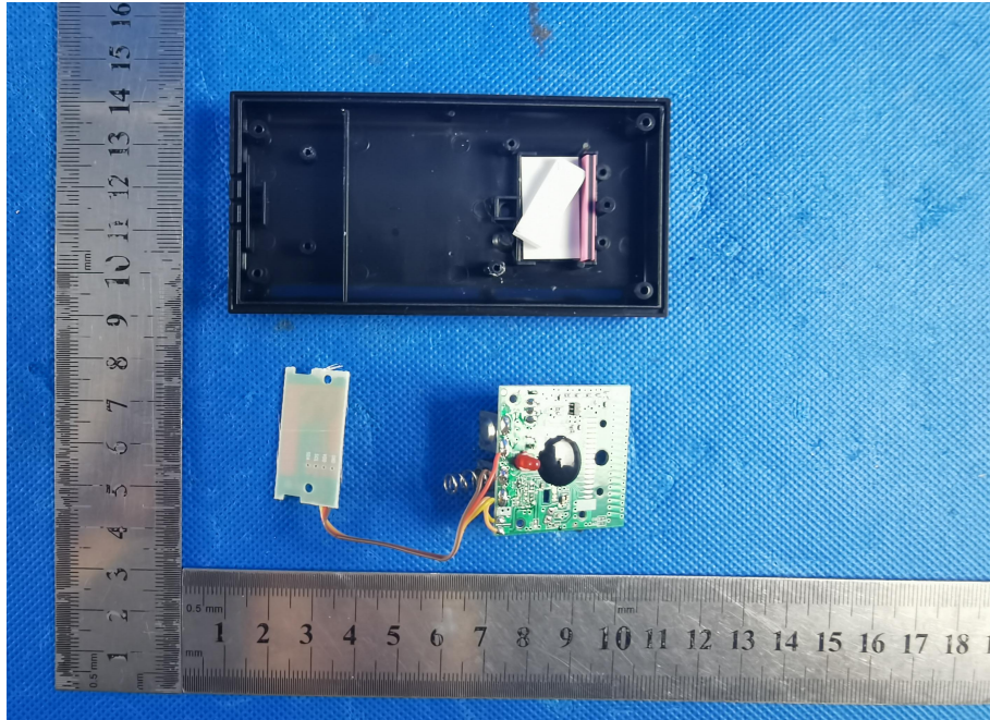
INTERNAL VIEW OF EUT(Figure 1)
