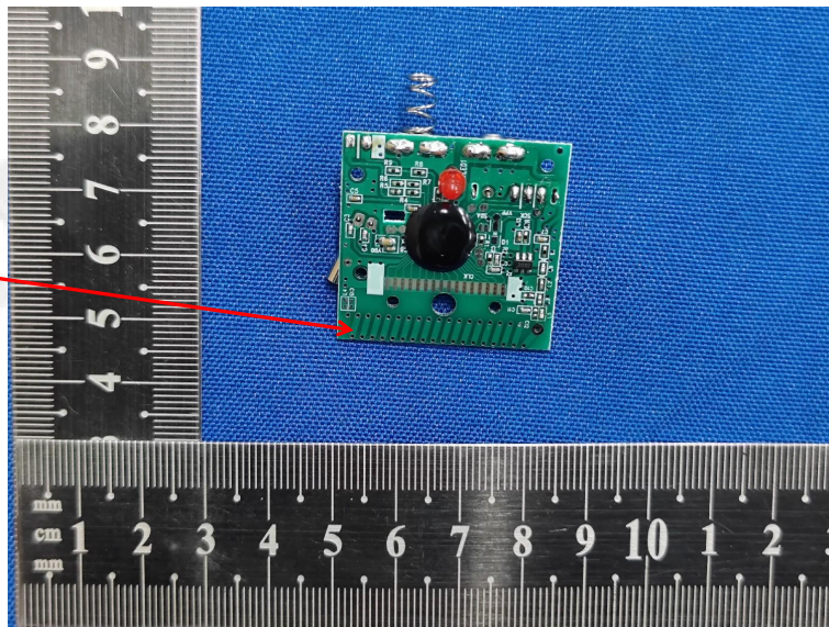
Transmitter antenna
