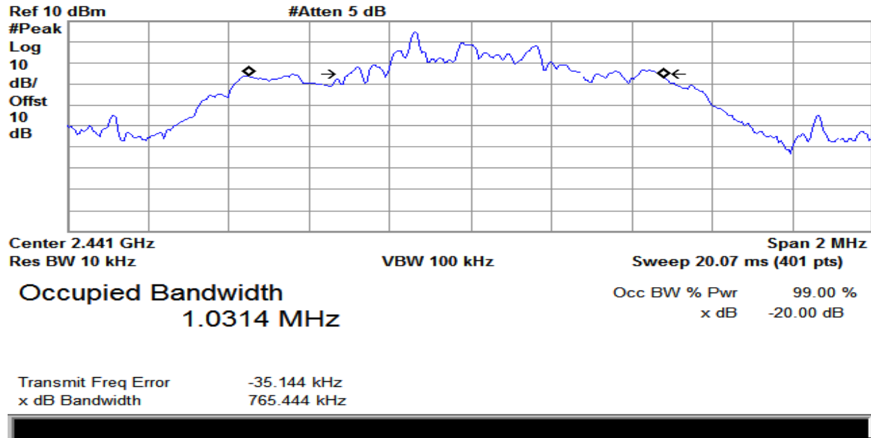
Plot 7 – Middle Channel – 20dB BW ( \pi/4 -DQPSK 2Mbps)
