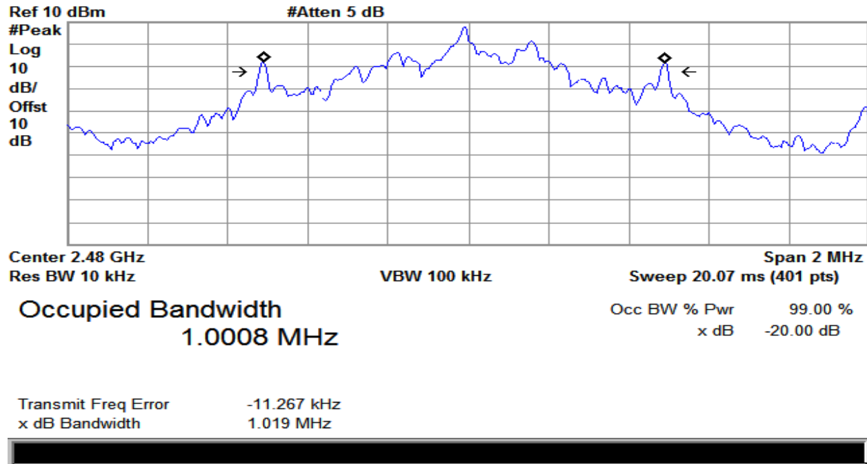
Plot 5 – Highest Channel – 20dB BW (GFSK 1Mbps)
