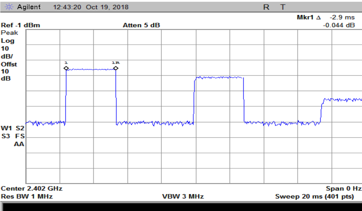
Plot 37 – Dwell Time ( \pi/4 -DQPSK)
