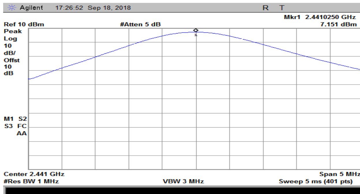
Plot 13 – Output Power – Middle Channel
