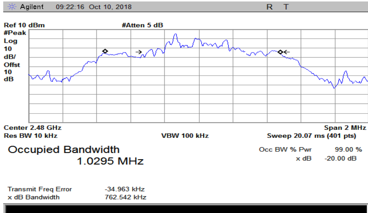
Plot 8 – Highest Channel – 20dB BW ( \pi/4 -DQPSK 2Mbps)
