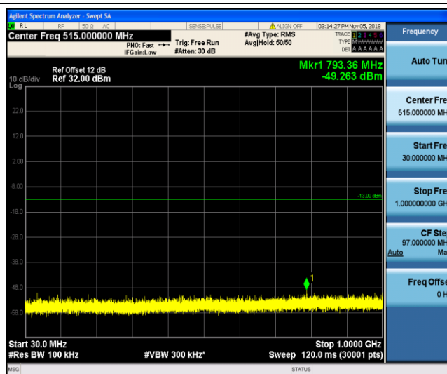
Band2 3MHz 16QAM 18615 1RB#0
