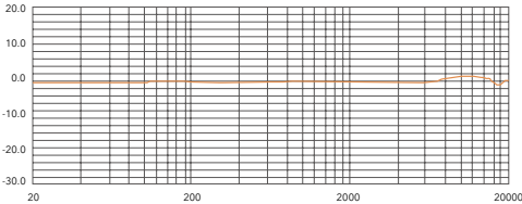
Frequency Response
