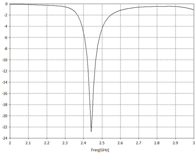
Antenna return loss:
