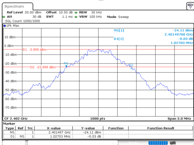
GFSK_Low
