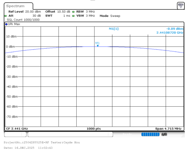
GFSK_Middle
