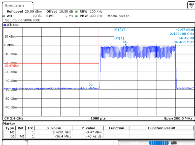
GFSK_Hopping_Lower
