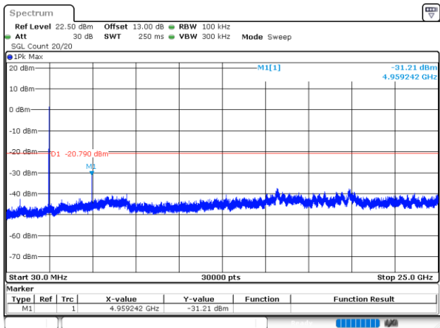
GFSK_High
