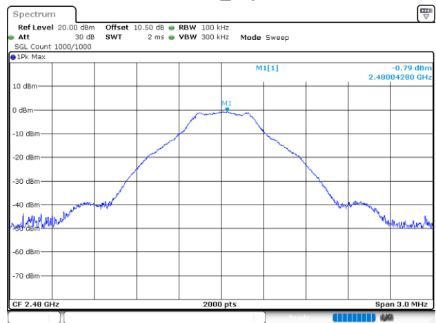
GFSK_High
