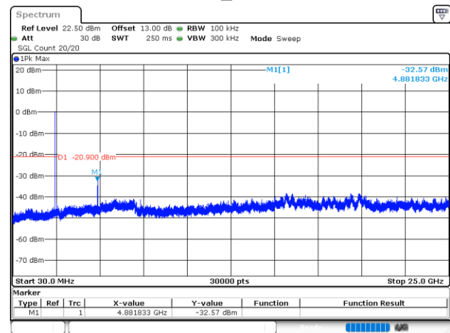
GFSK_Middle
