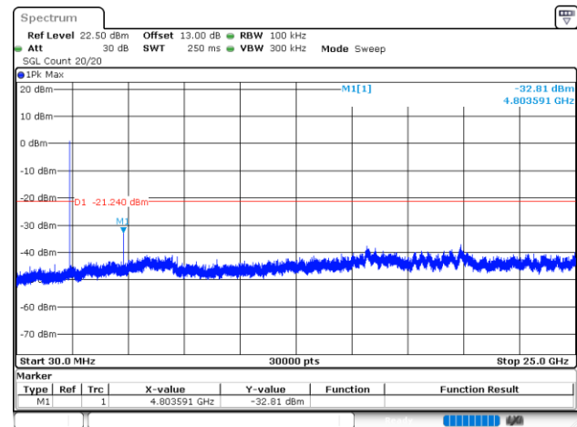
GFSK_Low
