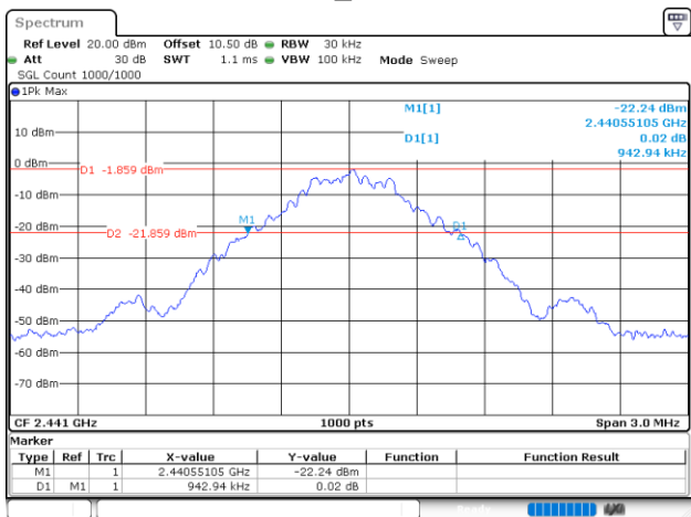
GFSK_Middle
