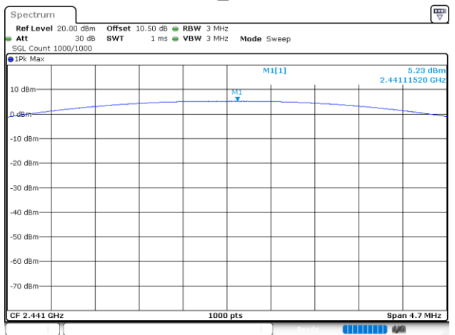
GFSK_Middle
