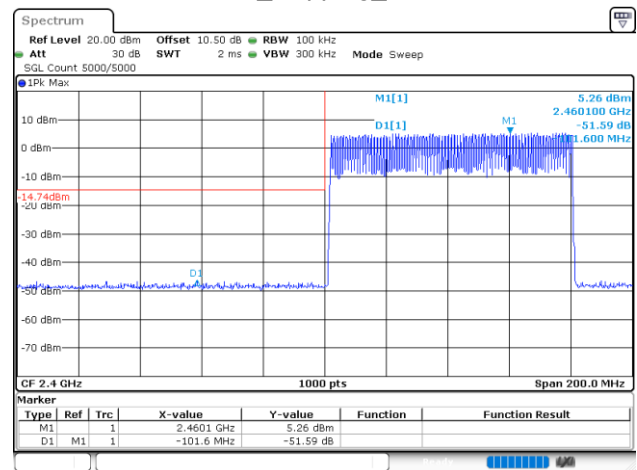
GFSK_Hopping_Lower
