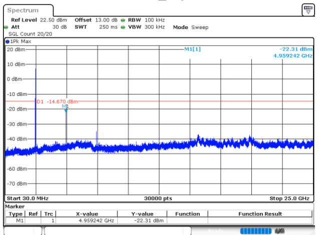
GFSK_High
