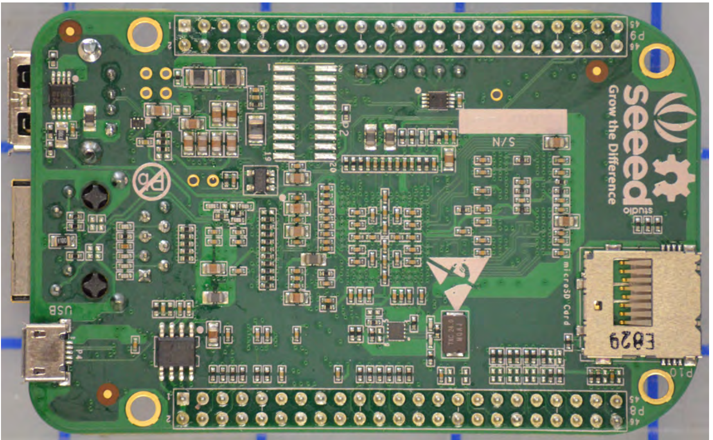
Processor board bottom view
