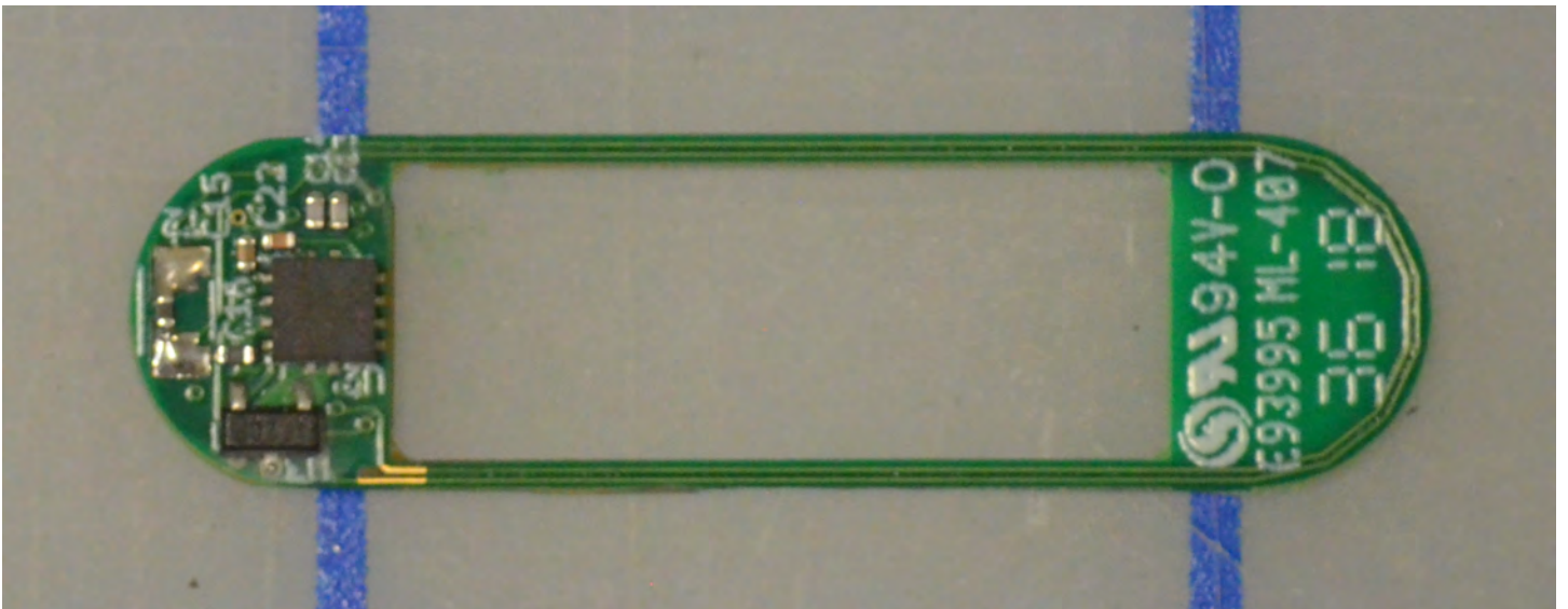
Stirbar board bottom view
