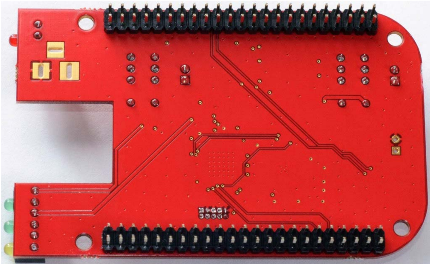
Figure E20.2 – External Photo – Radio Cape Module Bottom
