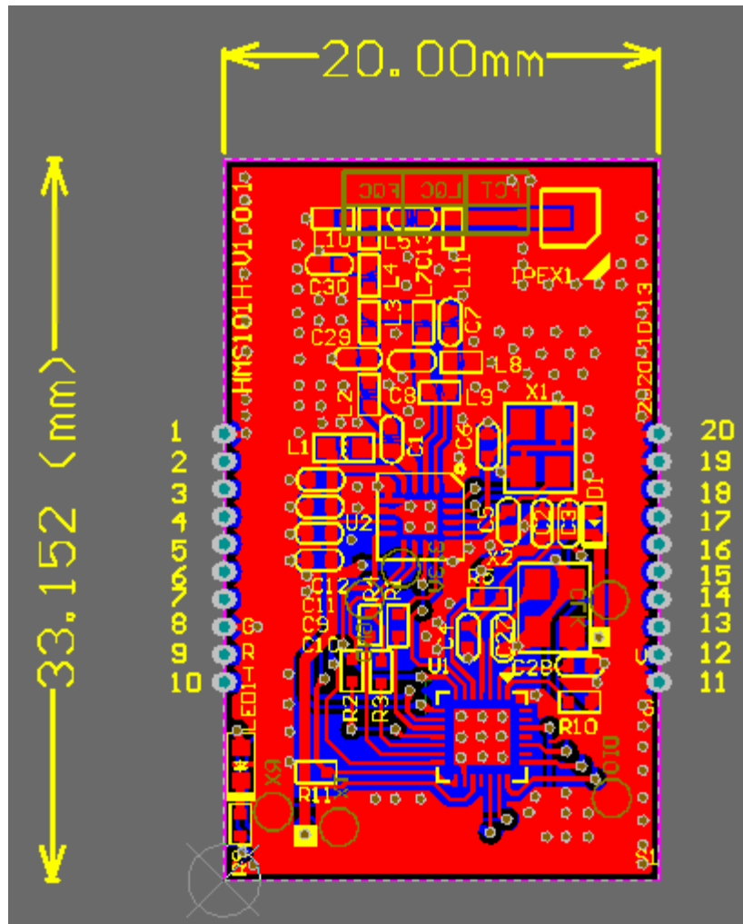
Figure 1 HMS101 dimensions
