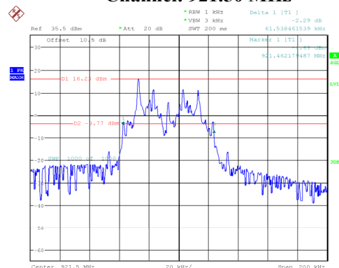
Channel: 921.50 MHz
