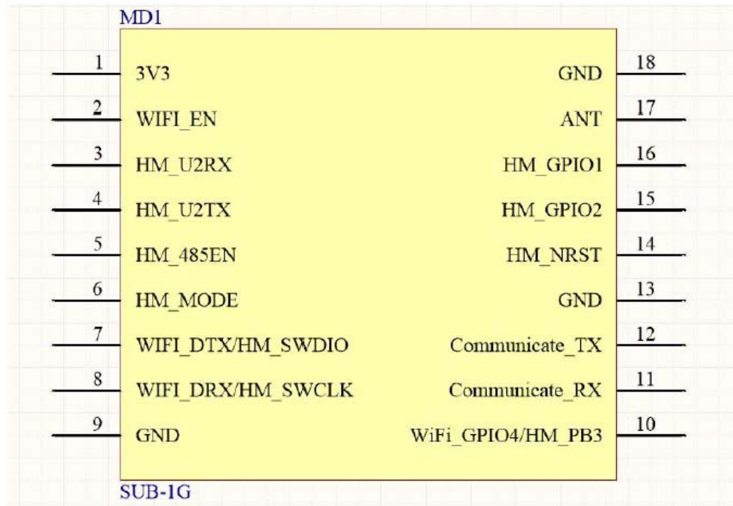
Figure 3-1: Top View Pinout Diagram
