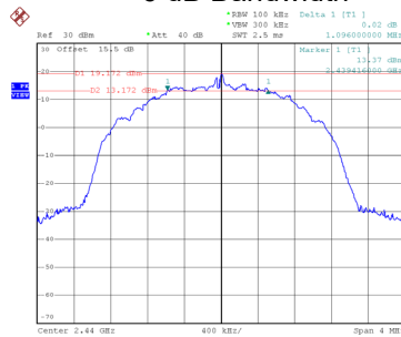
CH18 6 dB Bandwidth
