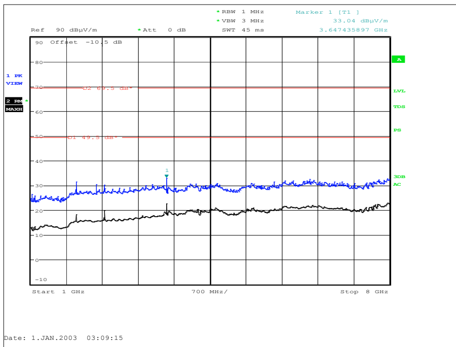
Figure 4 - Graphical Results - 1 GHz to 8 GHz Combined Polarity - EUT Orientation: X
