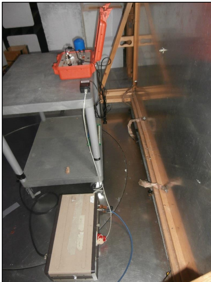
Figure 11 – Conducted Disturbance at Mains Terminals
