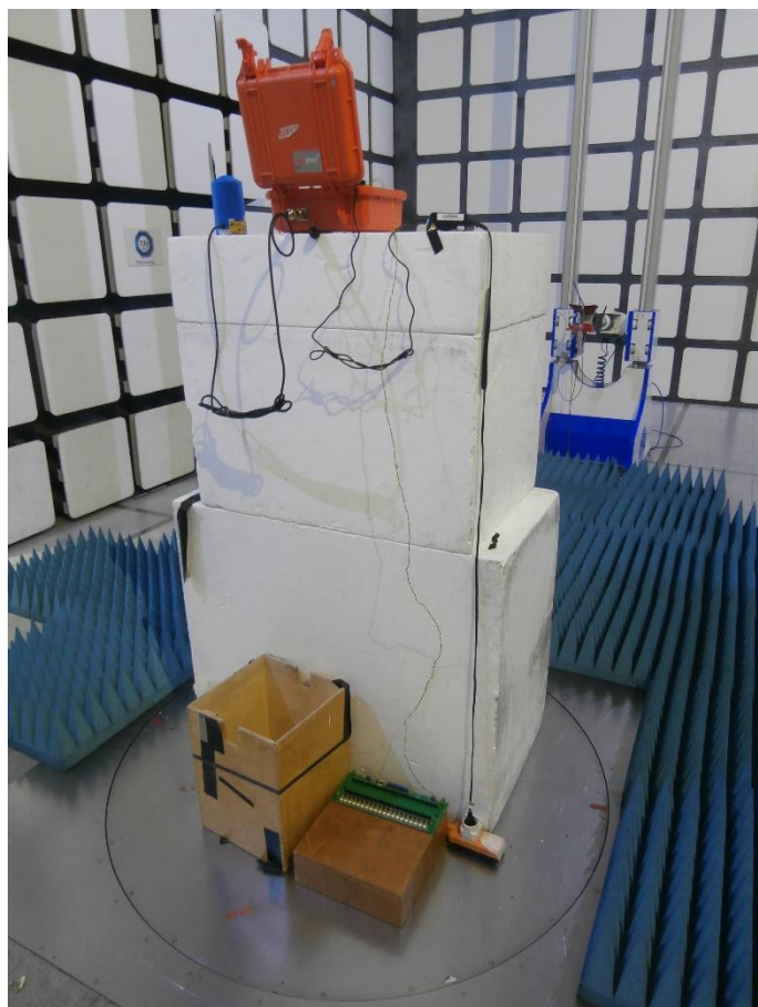
Figure 28 - Field Strength of Emissions - 1 GHz to 18 GHz
