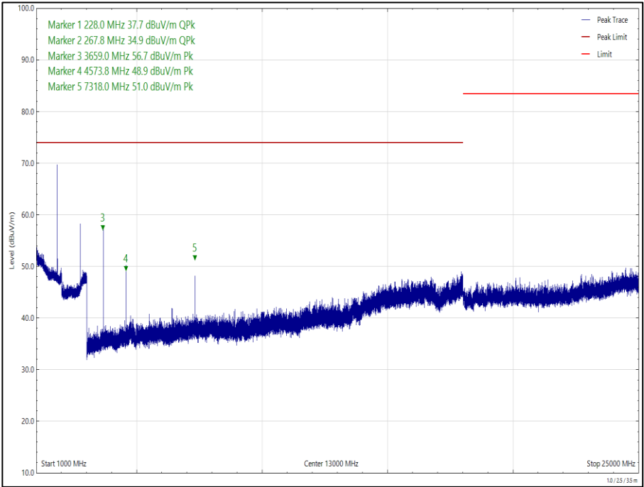
Figure 15 - 914.74 MHz - 1 GHz to 25 GHz, Polarity: Horizontal, EUT Orientation: Z, Peak
