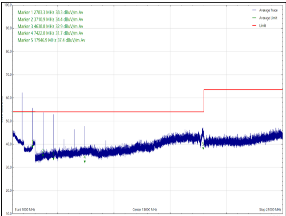
Figure 27 - 927.74 MHz, 1 GHz to 25 GHz, Vertical, Z Orientation, Average
