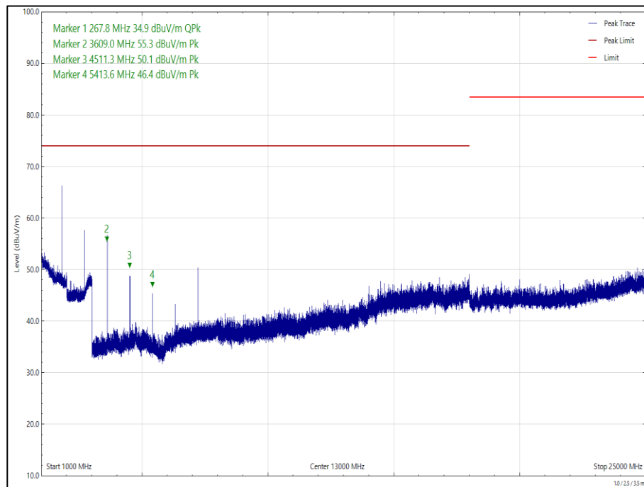
Figure 9 - 902.26 MHz, 1 GHz to 25 GHz, Horizontal, Z Orientation: - Peak
