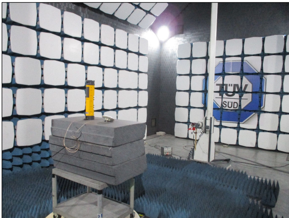
Figure 34 - Test Setup - 1 GHz to 18 GHz
