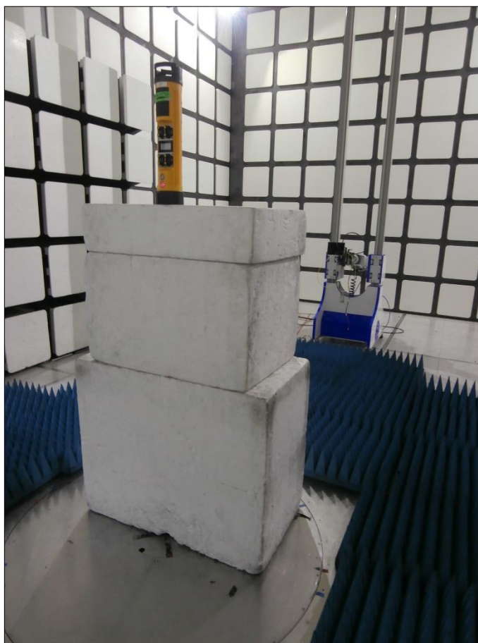
Figure 21 - Test Setup - 1 GHz to 1 GHz
