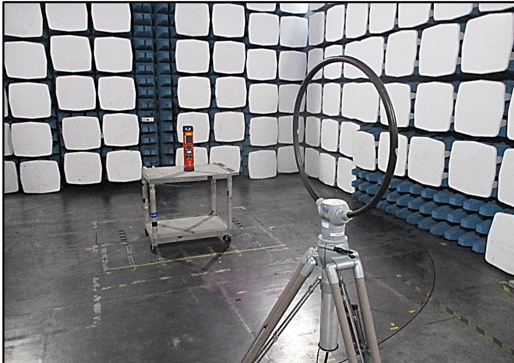
Figure 6 - Test Setup
