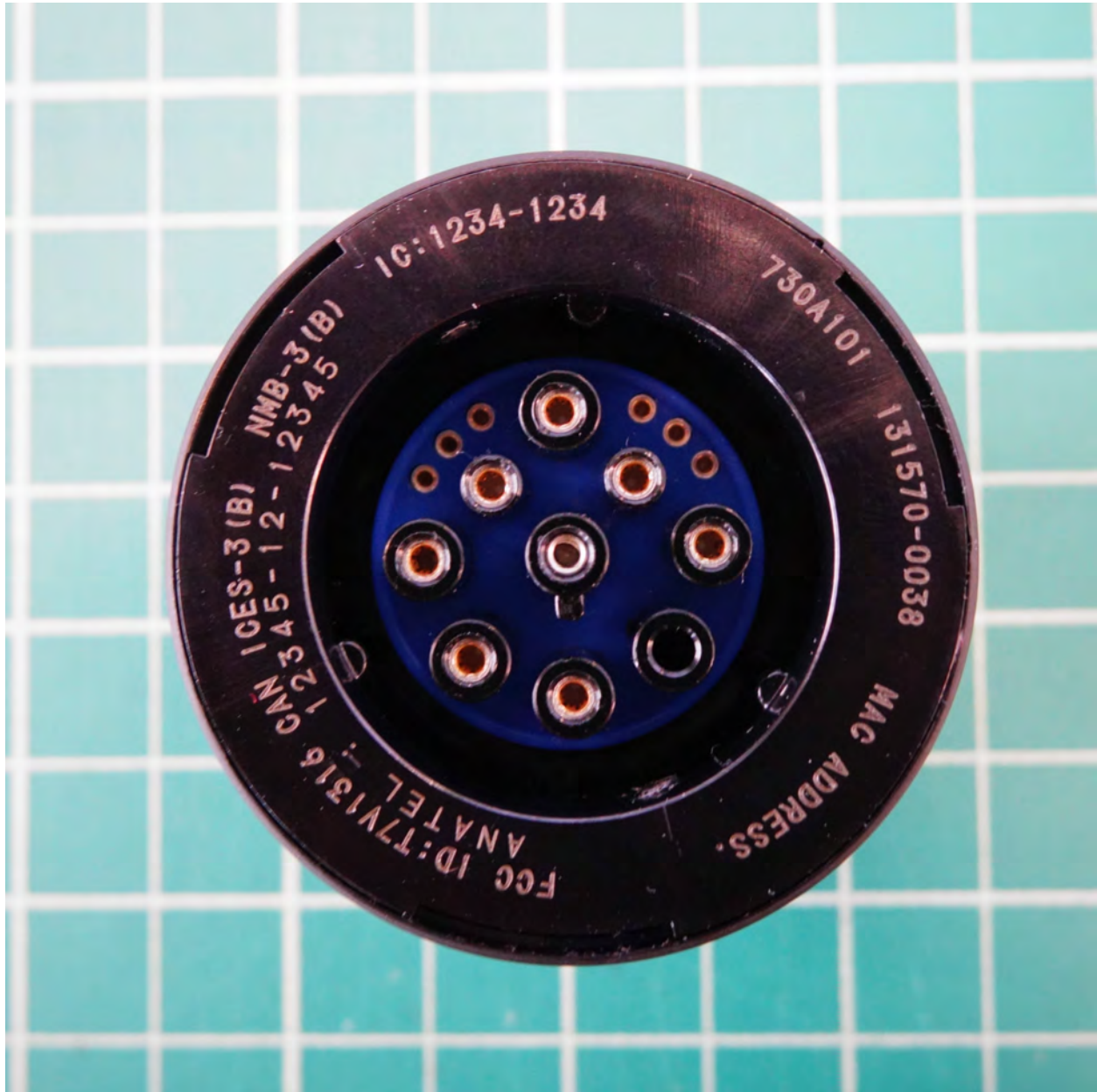
Picture 3 - Detailed view of FieldView Drive 2 enclosure bottom, including view of the J1939 connector and prototype markings. These markings do not reflect what will be used on the final product.
