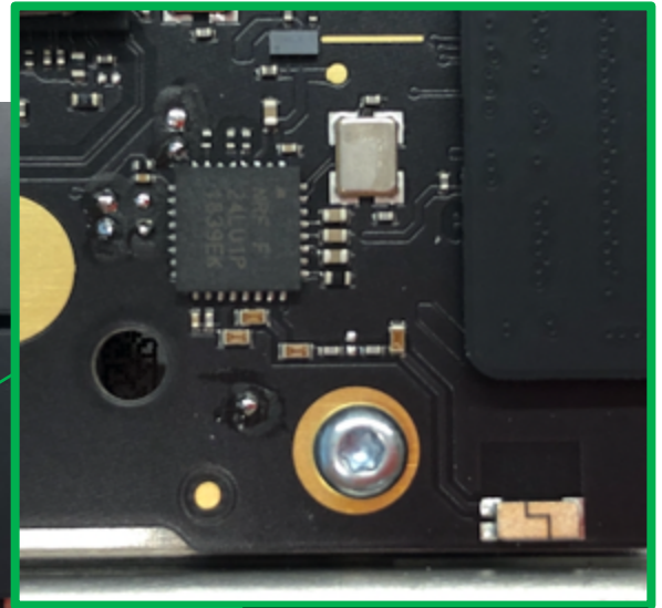
Radio circuit U2001 and antenna A2001 location
