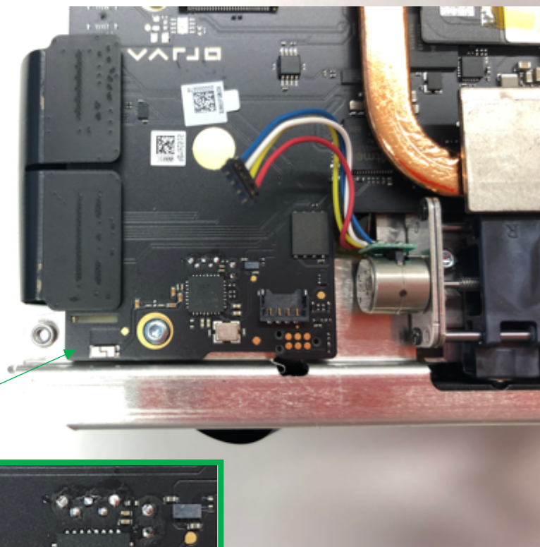
Radio circuit U2000 and antenna A2000 location
