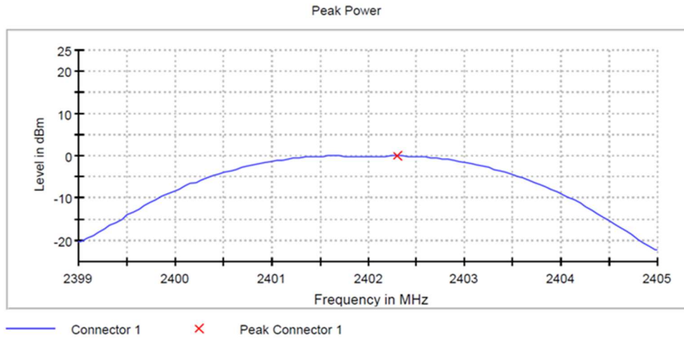
Figure 4: Conducted power, Channel LOW (left antenna)
