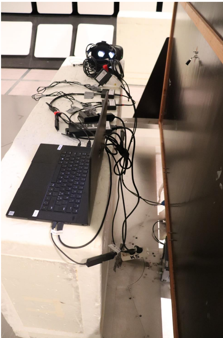
Photograph 7. Conducted Emission, CNTX
