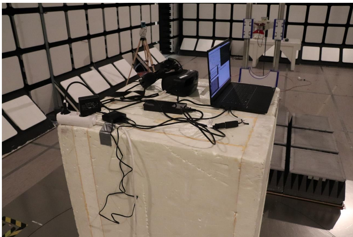
Photograph 4: The EUT arrangement during Radiated Emissions (1 - 26.5 GHz)
