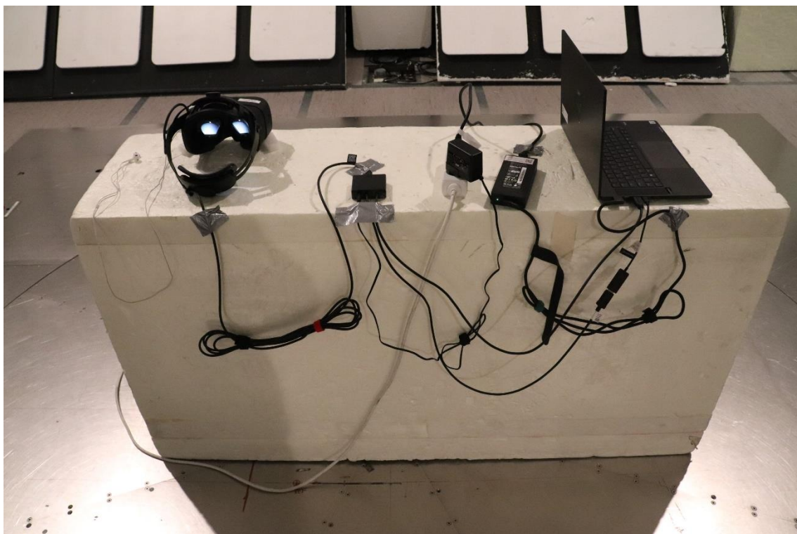
Photograph 1. The EUT arrangement during Radiated Emissions (9 kHz – 1000 MHz)
