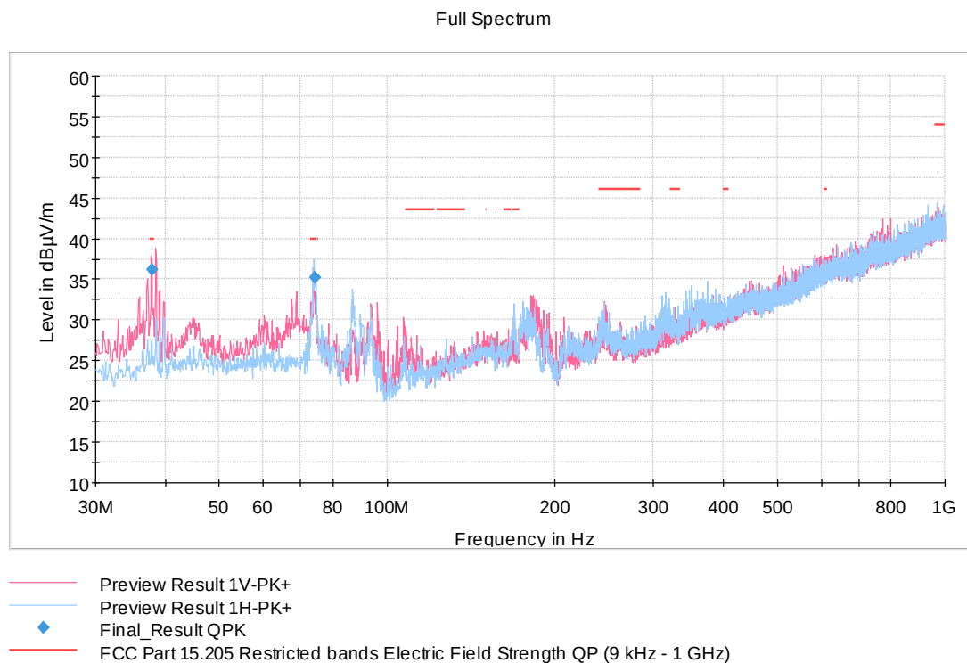
Figure 16: Unwanted emissions 30 – 1000 MHz (ch. config. 3)
