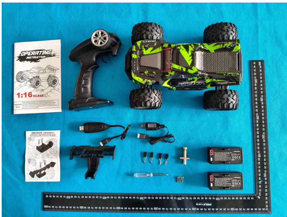
External Photo 2
