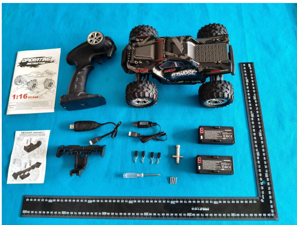
External Photo 6
