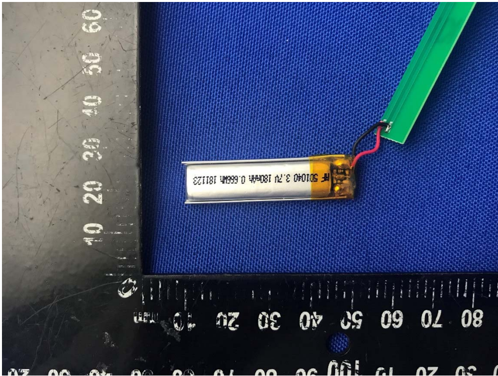
Battery Photo (FRONT) (#2)
