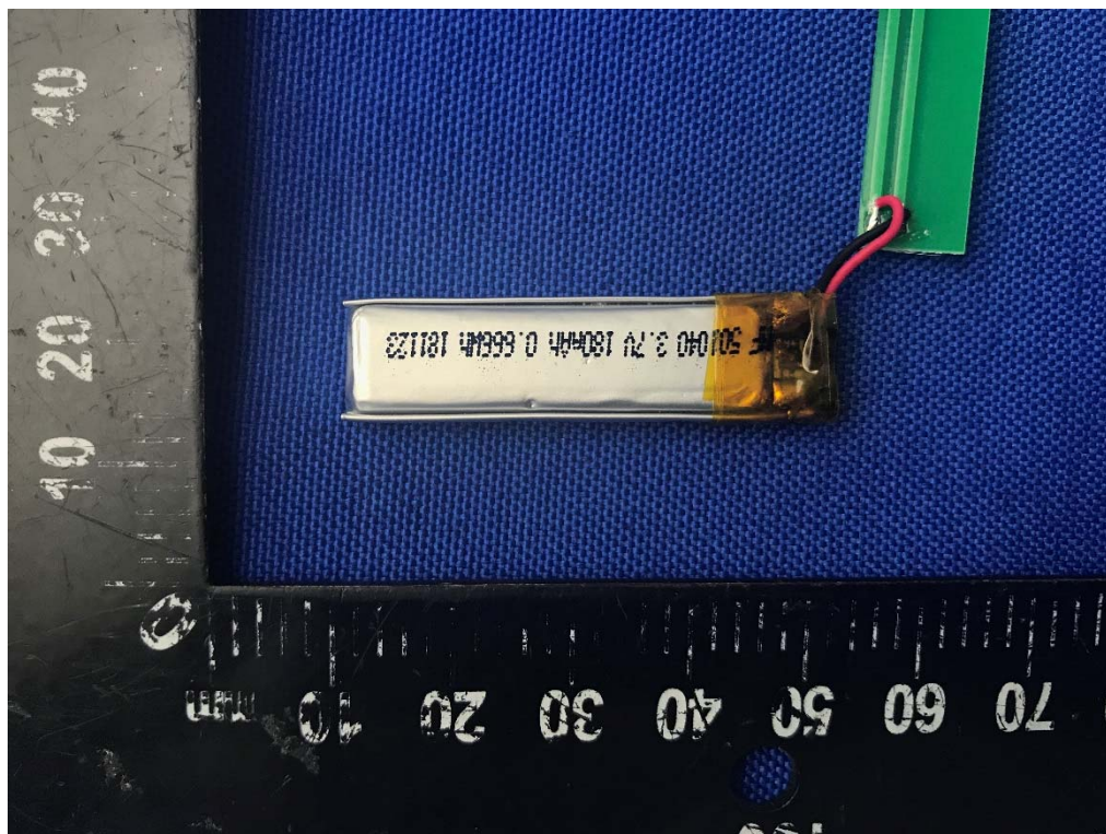
Battery Photo (FRONT) (#1)
