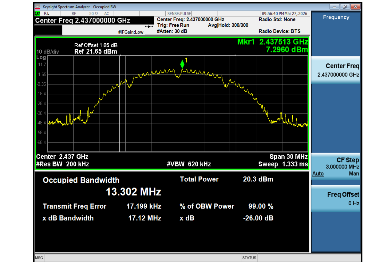
OBW NVNT b 2437MHz Ant1
