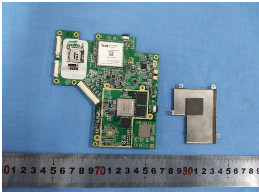
EUT – Mainboard Top Uncovered View
