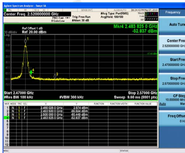
Right bandedge
