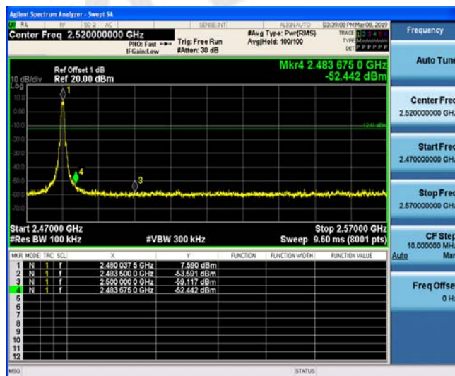
Right bandedge
