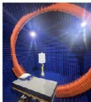
Testing 3D microwave darkroom(6m*6m*6m)
