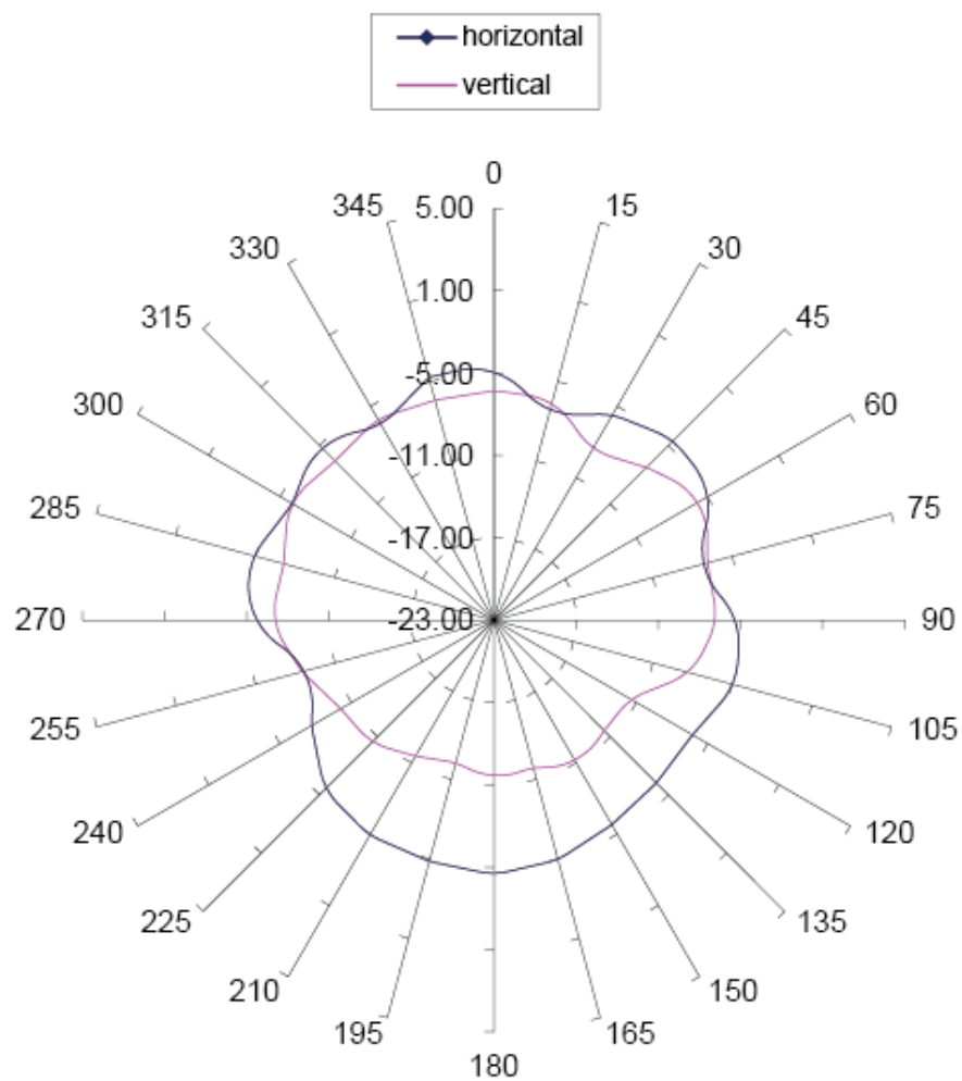
Fixed Part, Antenna 0, Horizontal and Vertical diag.
