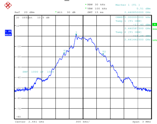
DH1_Middle 0.855MHz
