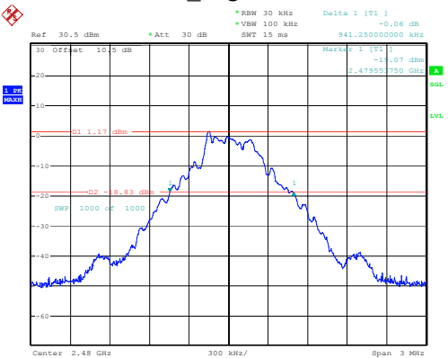
DH1_High 0.941MHz
