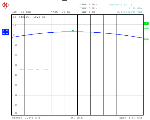
DH1_Middle 2.98dBm
