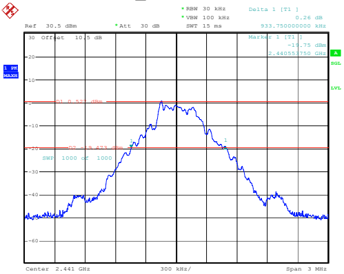
DH1_Middle 0.934MHz
