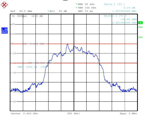
2DH1_Low 1.208MHz
