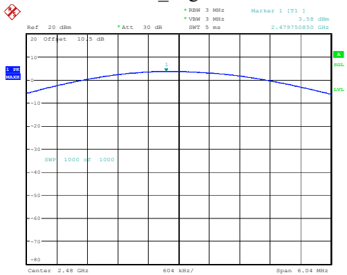
2DH1_High 3.58dBm
