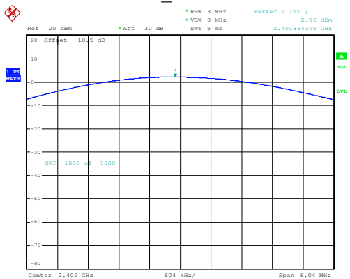
2DH1_Low 2.06dBm
