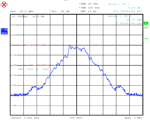
DH1_Low 0.934MHz
