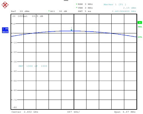
DH1_Low 2.15dBm
