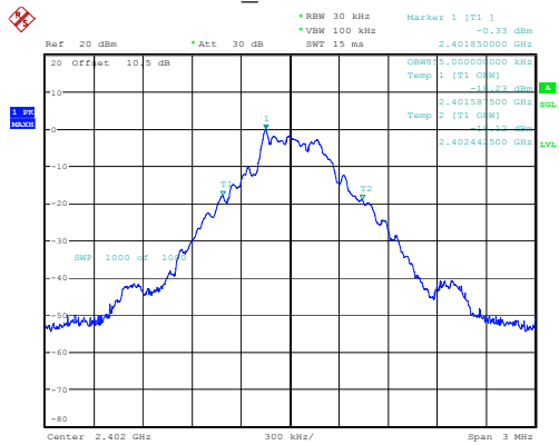
DH1_Low 0.855MHz
