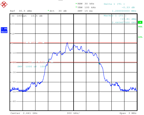
2DH1_Middle 1.200MHz
