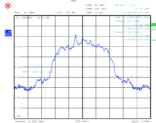
2DH1_Low 1.133MHz
