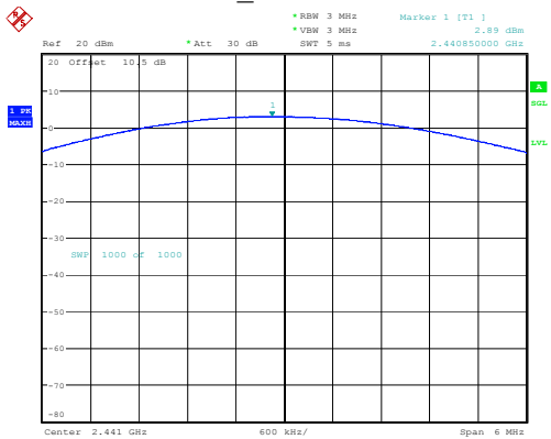
2DH1_Middle 2.89dBm
