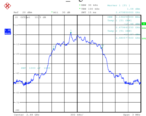
2DH1_High 1.136MHz
