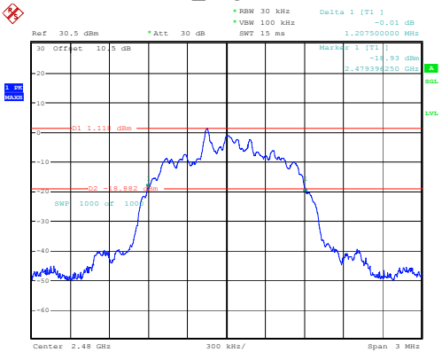
2DH1_High 1.208MHz
