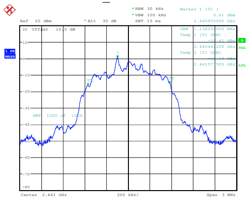
2DH1_Middle 1.136MHz
