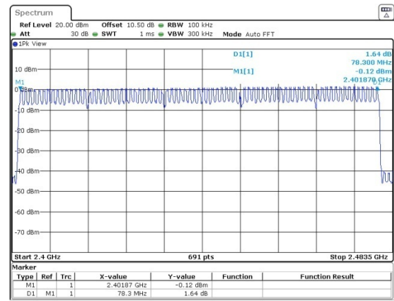
2DH1_Hopping 79
