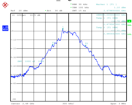
DH1_High 0.855MHz
