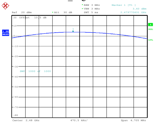
DH1_High 3.60dBm
