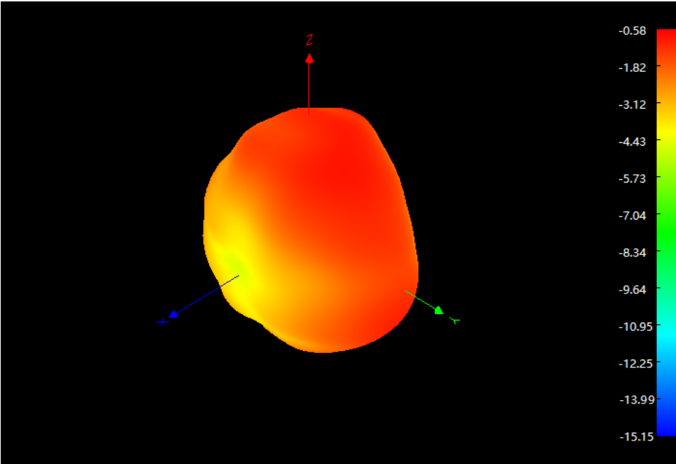
3D Radiation Pattern @ 2450 MHz
