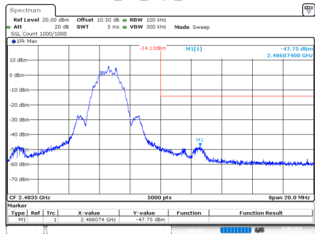
BLE_2M_High_Channel
