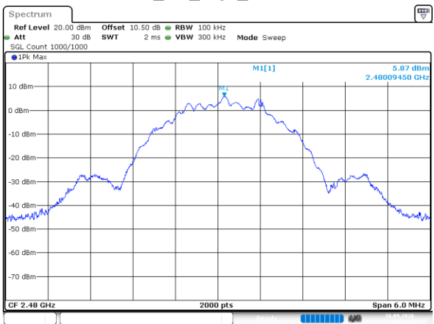
BLE_2M_High_Channel
