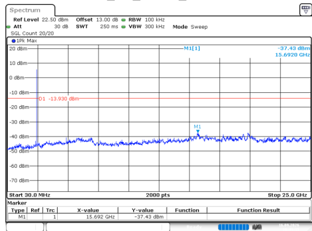
BLE_2M_Middle_Channel
