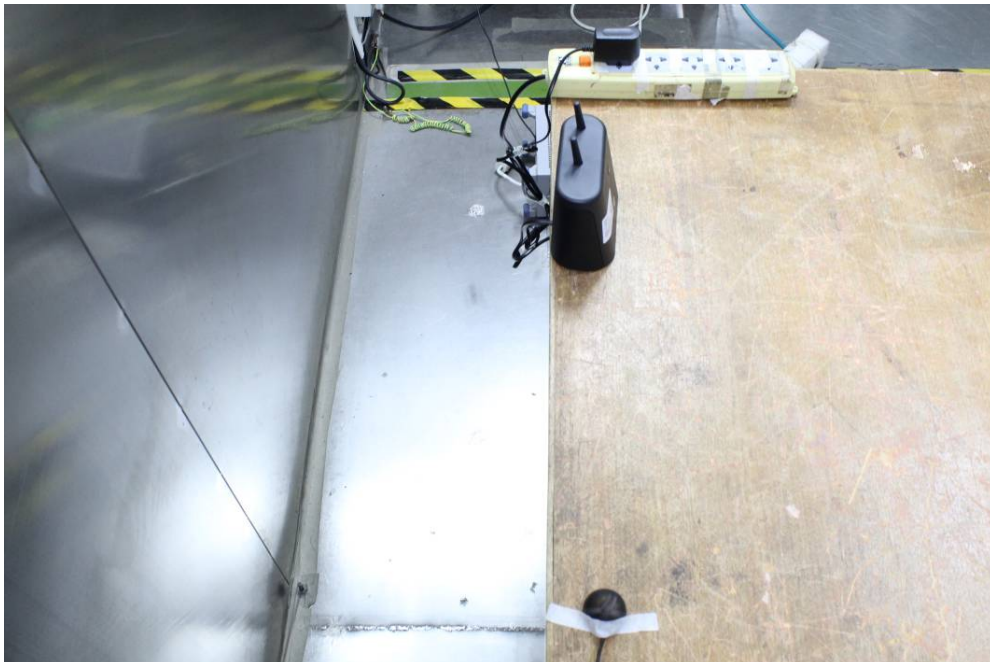
Conducted Emissions - Side View(Adapter 2)
