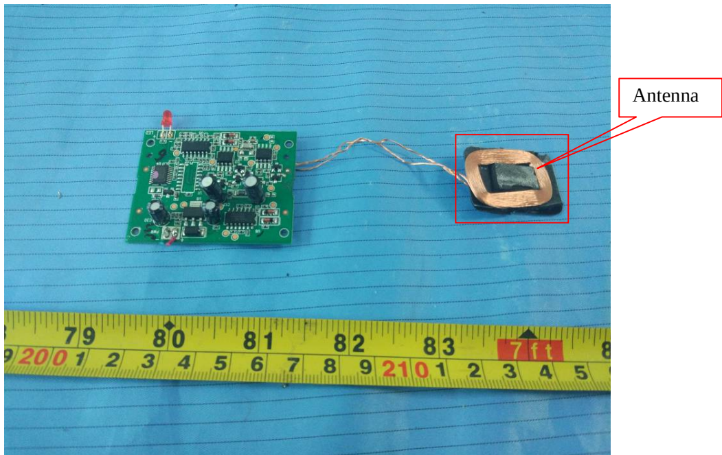
EUT – Main Board Front View
