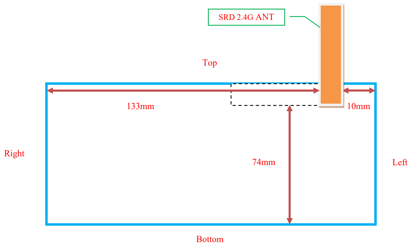
EUT Back View (Open)
