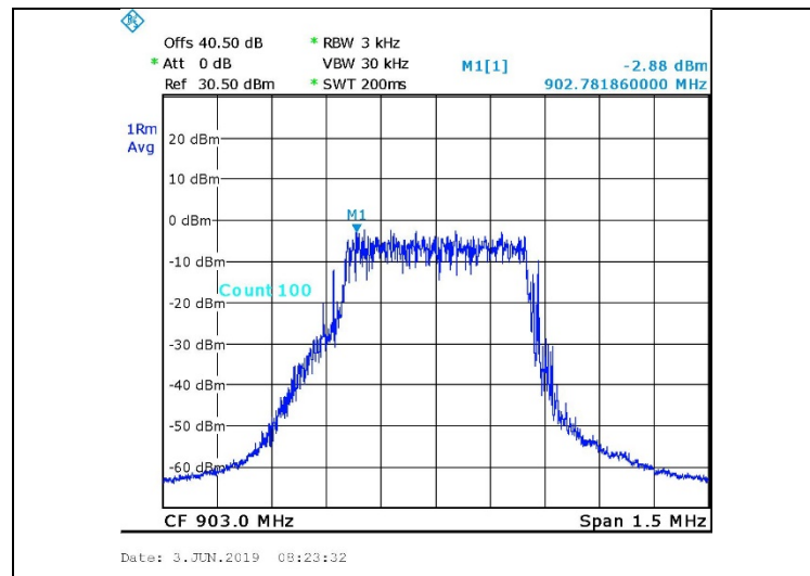
Figure 48. Low Channel, Main
