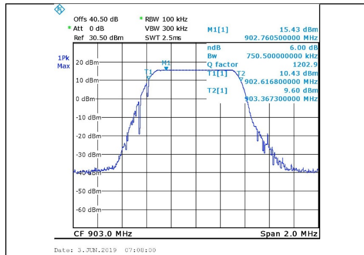
Figure 15. Low Channel, Main
