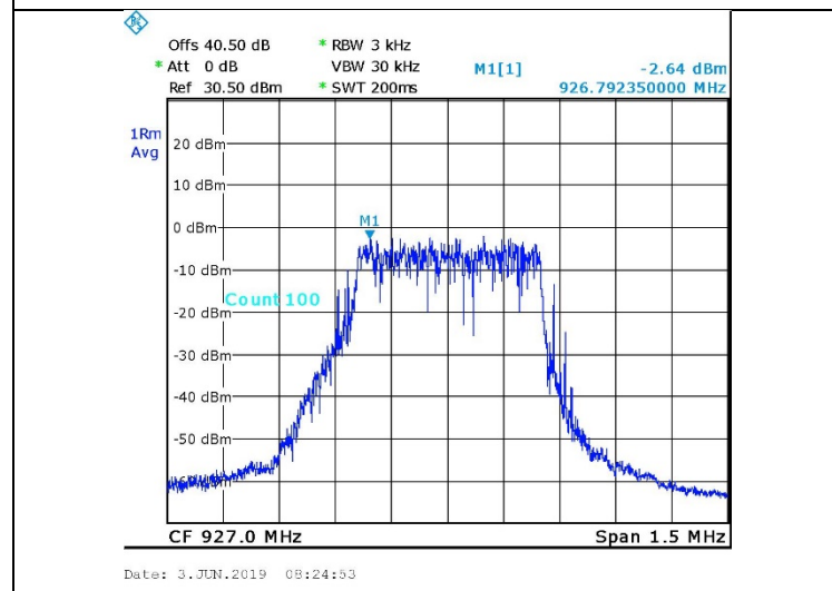
Figure 50. High Channel, Main
