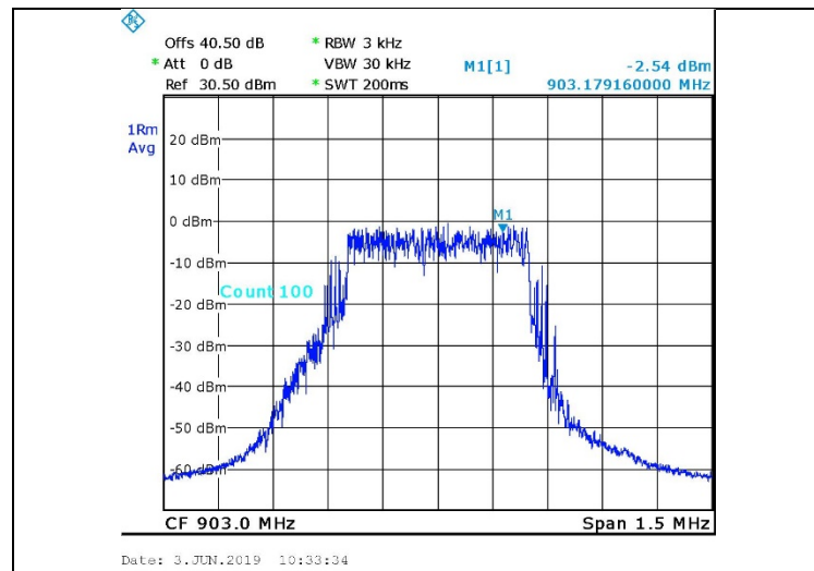
Figure 51. Low Channel, Secondary
