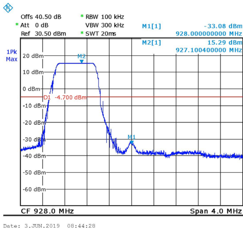
Figure 32 High Band Edge, Main
