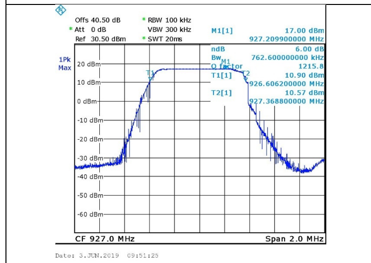
Figure 20. High Channel, Secondary
