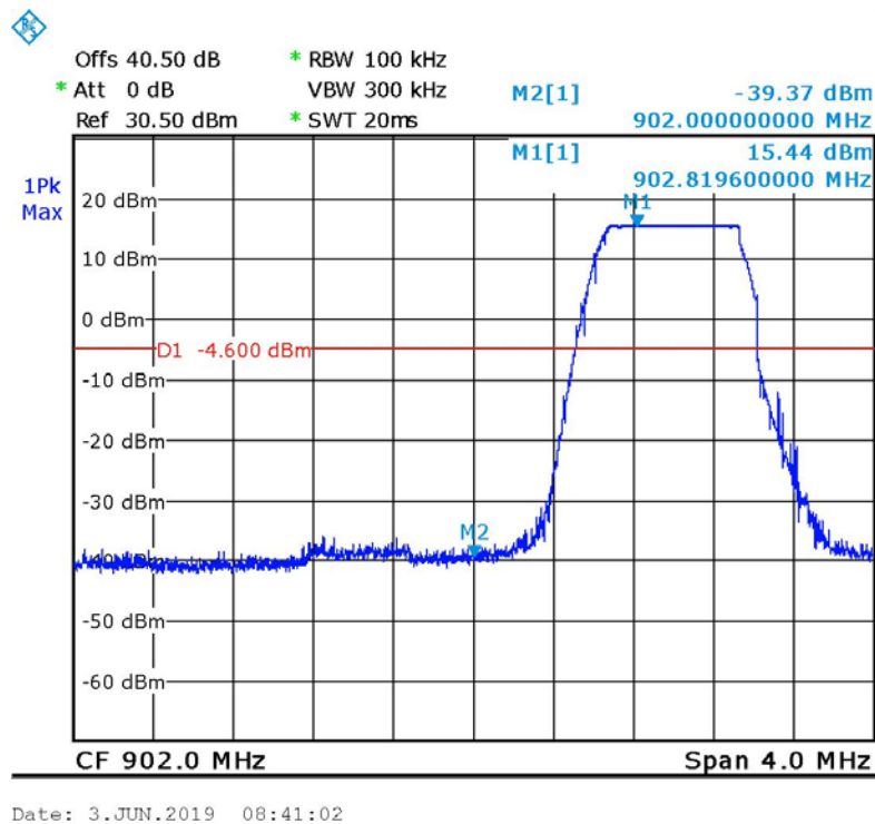
Figure 31 Low Band Edge, Main
