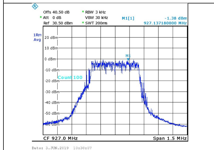
Figure 53. High Channel, Secondary
