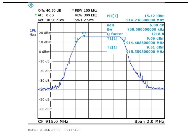
Figure 16. Mid Channel, Main
