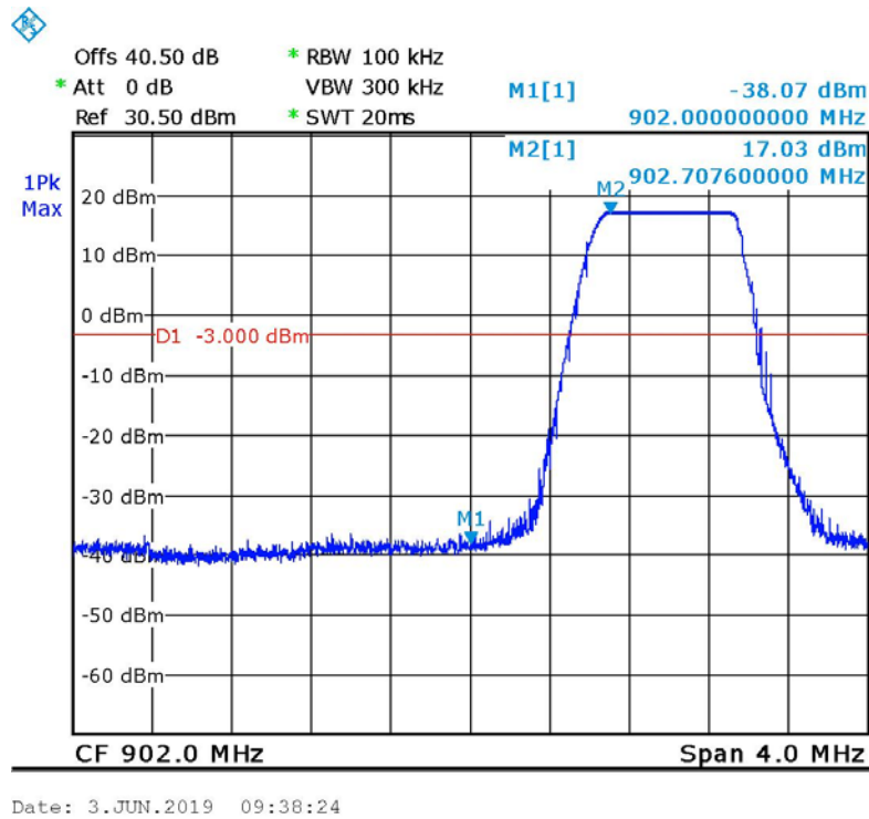
Figure 33 Low Band Edge, Secondary
