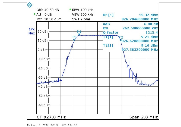
Figure 17. High Channel, Main
