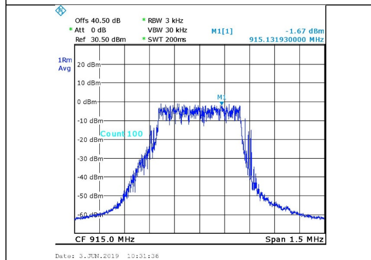
Figure 52. Mid Channel, Secondary
