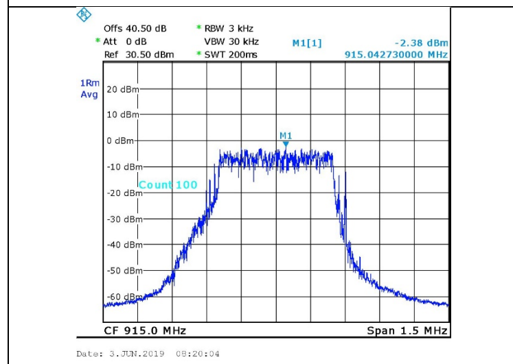
Figure 49. Mid Channel, Main
