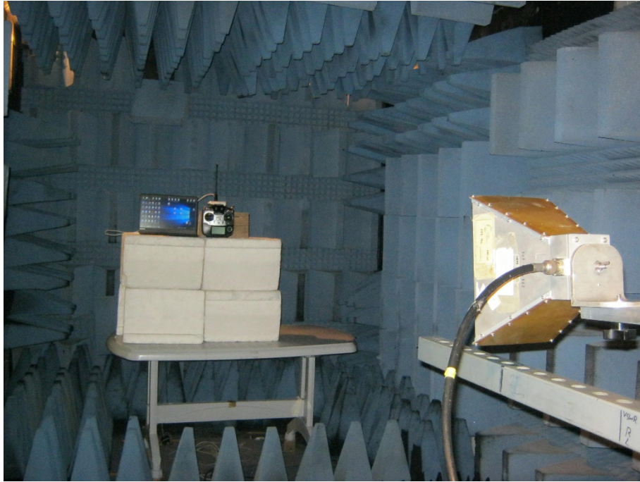
Radiated Emission Test, 1-10GHz
