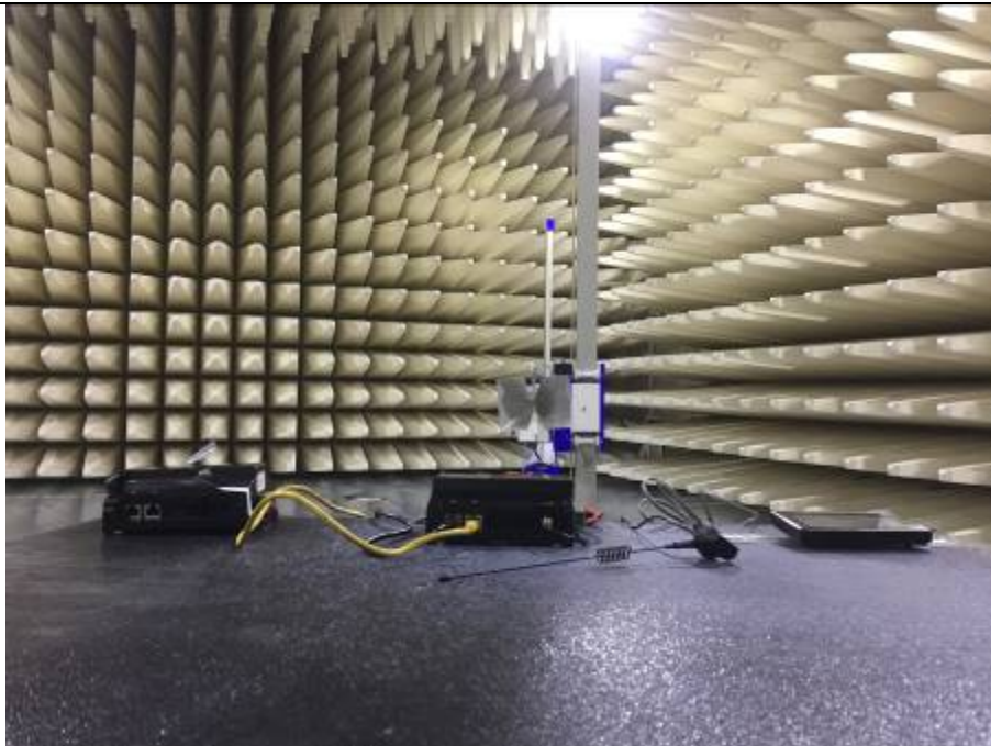
Spurious Radiated Emissions Test setup (above 1GHz) 1.5m
