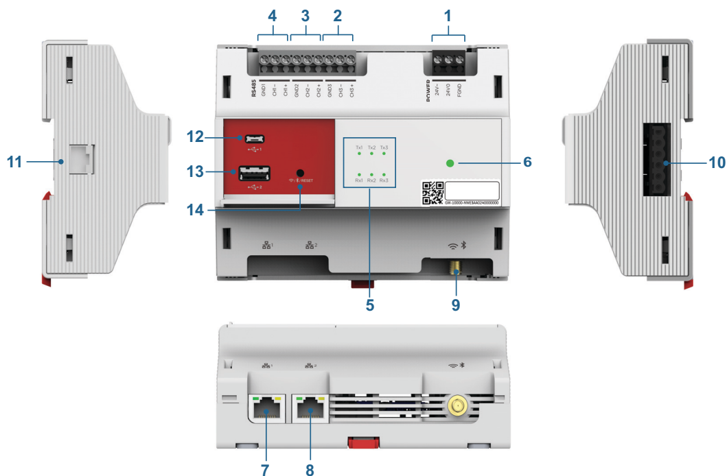
Fig. 1. GW-1000-WE/GW-1000-NWE Gateway
