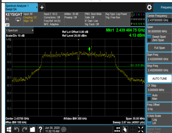
802.11g,2437MHz,Ant1,Plot 1,Reference Level
