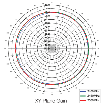
XY-Plane Gain
