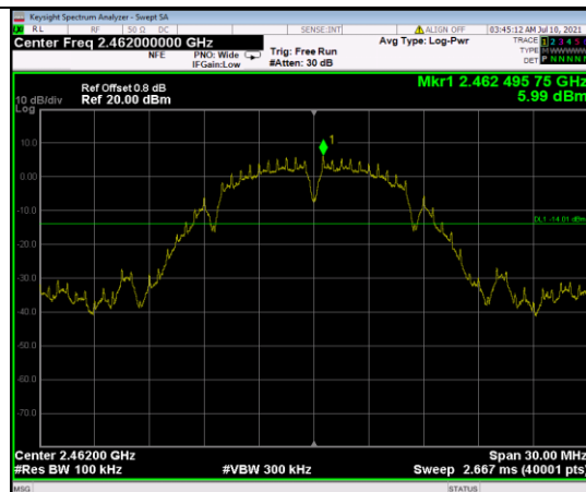
802.11b,2462MHz,Ant0,Plot 1,Reference Level
